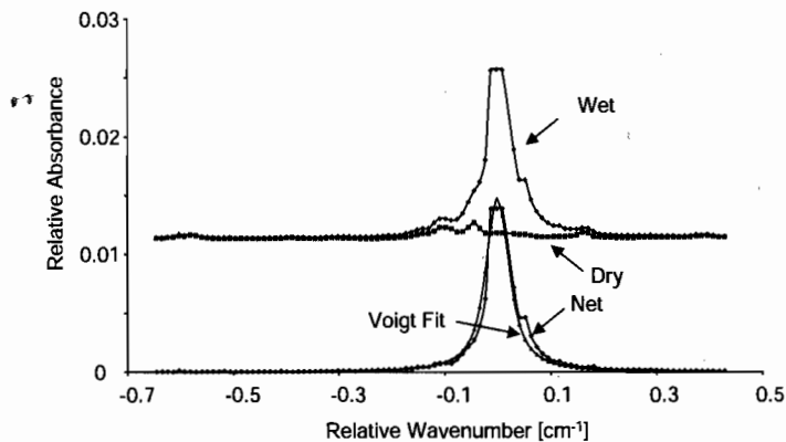
FIG. 4. Measured spectra and Voigt fit of the 1392.5 nm H_2O line. 829 nmol mol ^{-1} of H_2O in PH_3 at a total pressure of 12.6 kPa. For the Voigt fit, Gaussian full-width = 0.0208 cm ^{-1} , Lorentzian full-width = 0.04473 cm ^{-1} . Note: upper spectra are offset on the vertical scale for clarity.
