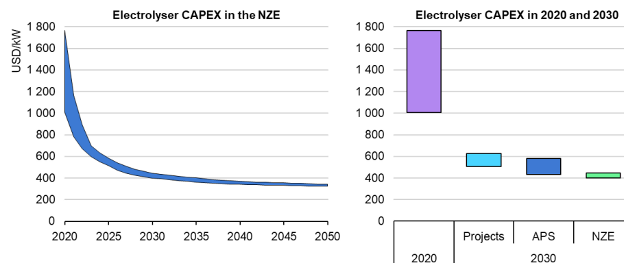
Evolution of electrolyser capital costs under the Projects case, Announced Pledges and Net zero Emissions scenarios
